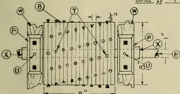
— DETAIL OF CYLINDER — SCALE - \frac{3}{16} " = 1"
